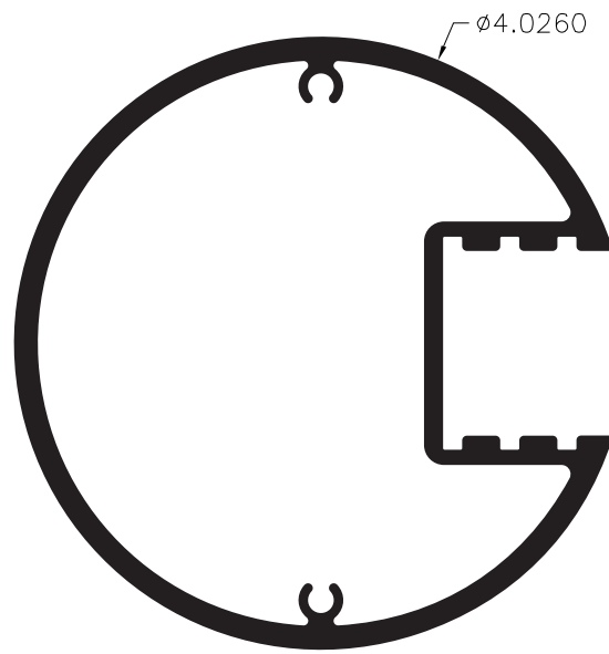
Series 4 Round Post Part #1337
